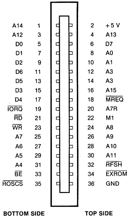
Fig. 6-2. DOCK connector.
